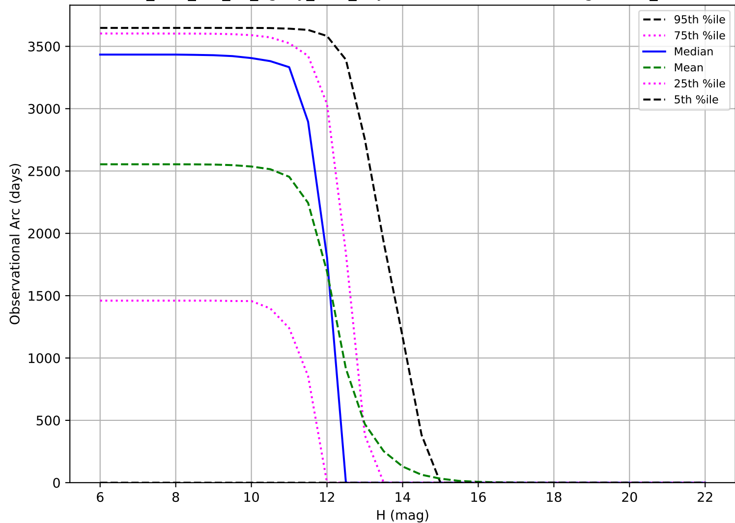
too_elab_r16_d3_ugrizy_v3.4_10yrs: Observational Arc Length OCC_r20
