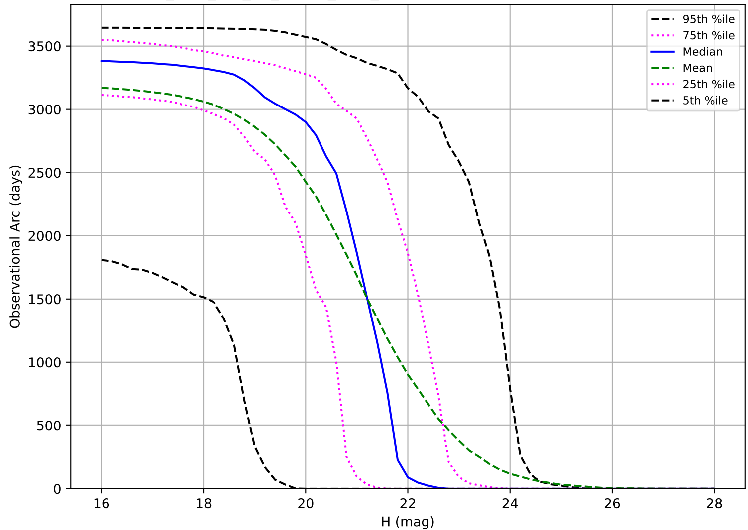
too_elab_r16_d3_ugrizy_v3.4_10yrs: Observational Arc Length NEO
