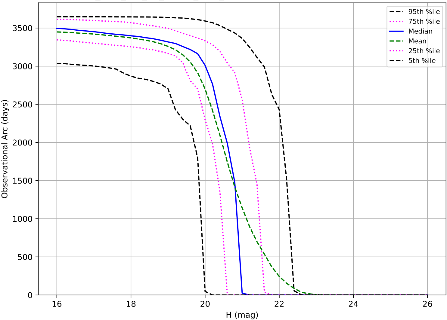
too_elab_r16_d3_ugrizy_v3.4_10yrs: Observational Arc Length MBA
