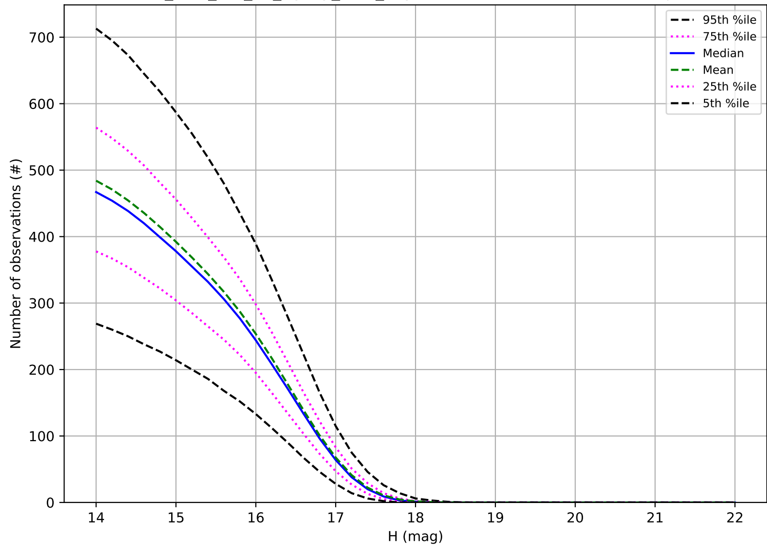
too_elab_r16_d3_ugrizy_v3.4_10yrs: Number of observations Trojan
