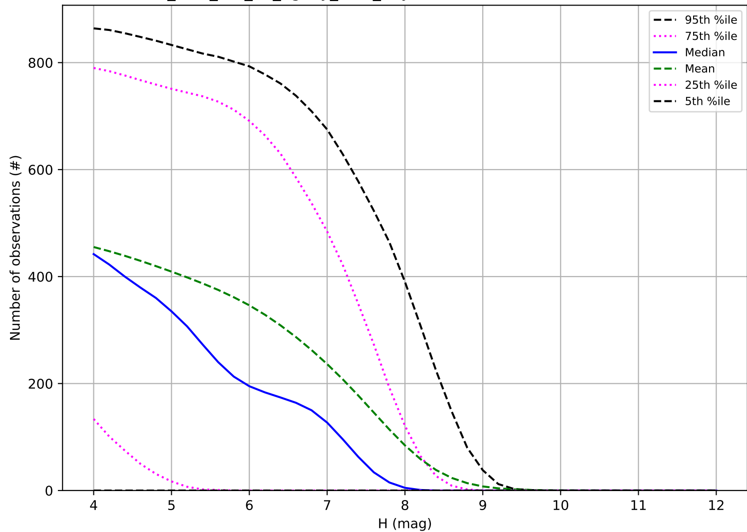
too_elab_r16_d3_ugrizy_v3.4_10yrs: Number of observations TNO
