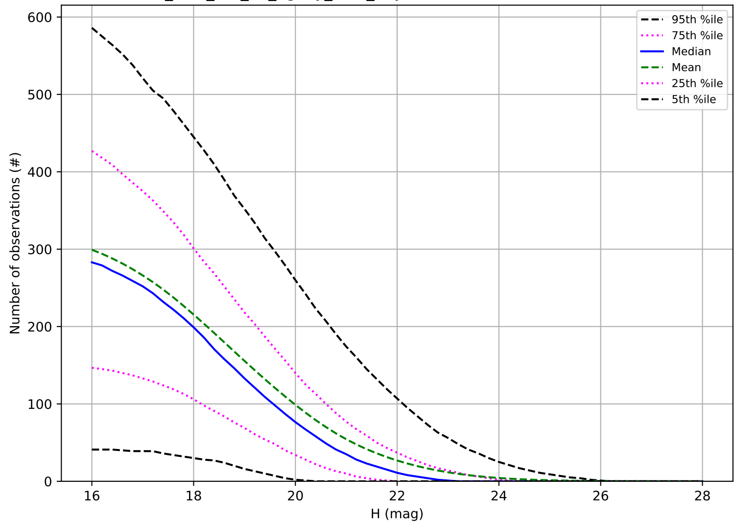
too_elab_r16_d3_ugrizy_v3.4_10yrs: Number of observations PHA
