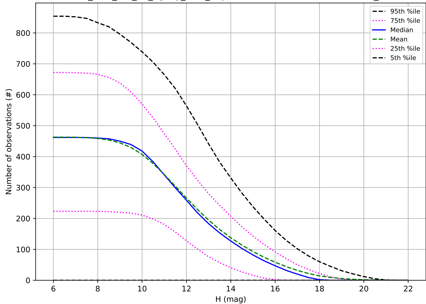
too_elab_r16_d3_ugrizy_v3.4_10yrs: Number of observations OCC_r5
