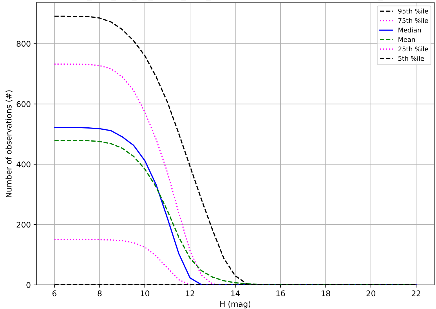
too_elab_r16_d3_ugrizy_v3.4_10yrs: Number of observations OCC_r20
