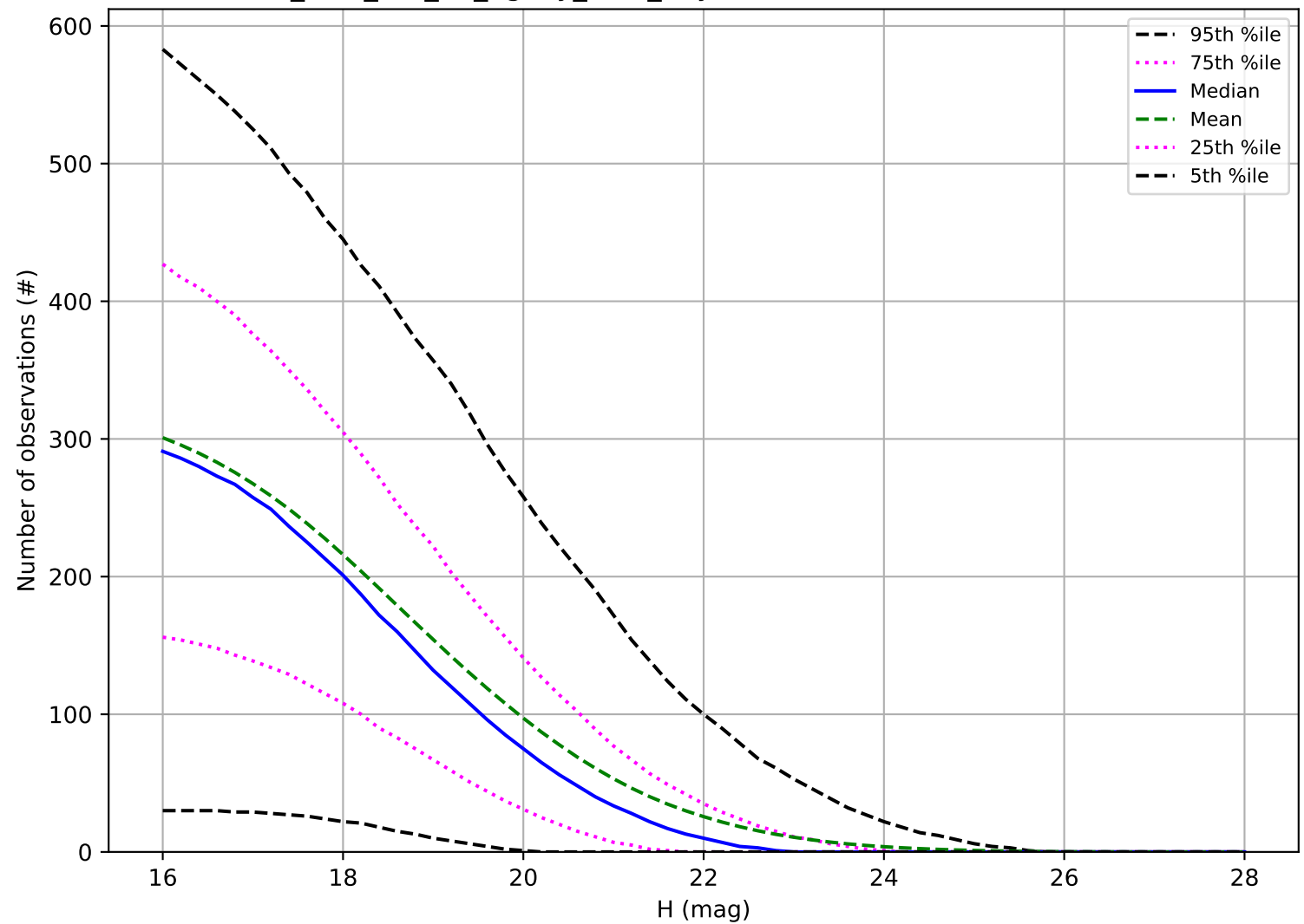
too_elab_r16_d3_ugrizy_v3.4_10yrs: Number of observations NEO
