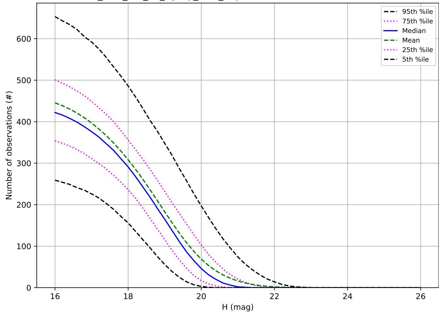
too_elab_r16_d3_ugrizy_v3.4_10yrs: Number of observations MBA
