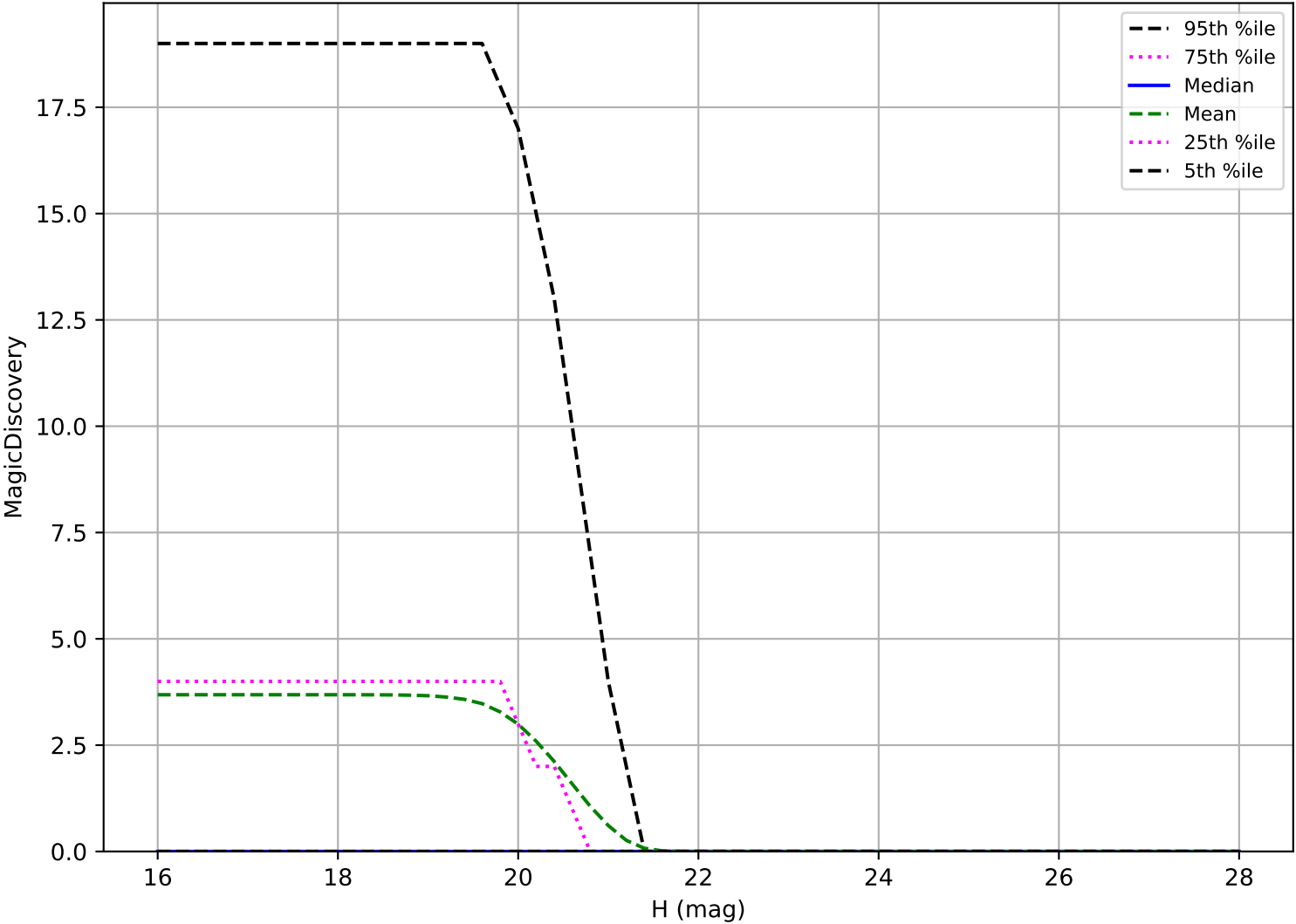
too_elab_r16_d3_ugrizy_v3.4_10yrs: Vatira 6 detections in 60 nights detection loss
