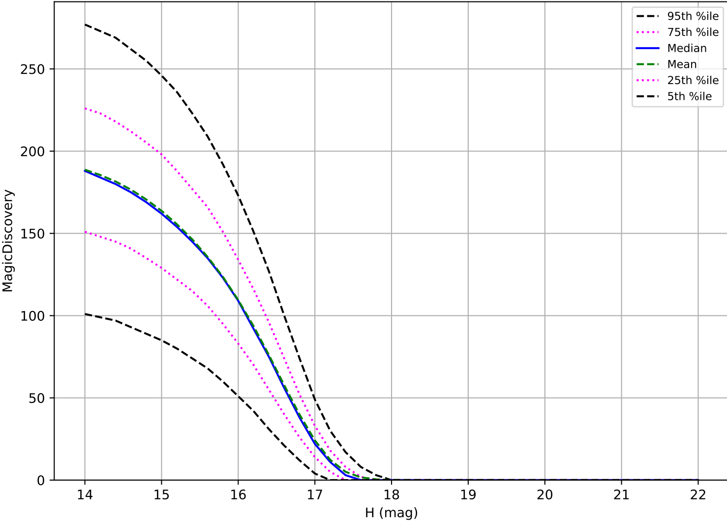
too_elab_r16_d3_ugrizy_v3.4_10yrs: Trojan 6 detections in 60 nights detection loss
