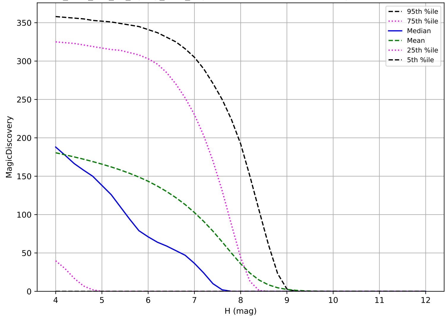
too_elab_r16_d3_ugrizy_v3.4_10yrs: TNO 6 detections in 60 nights detection loss
