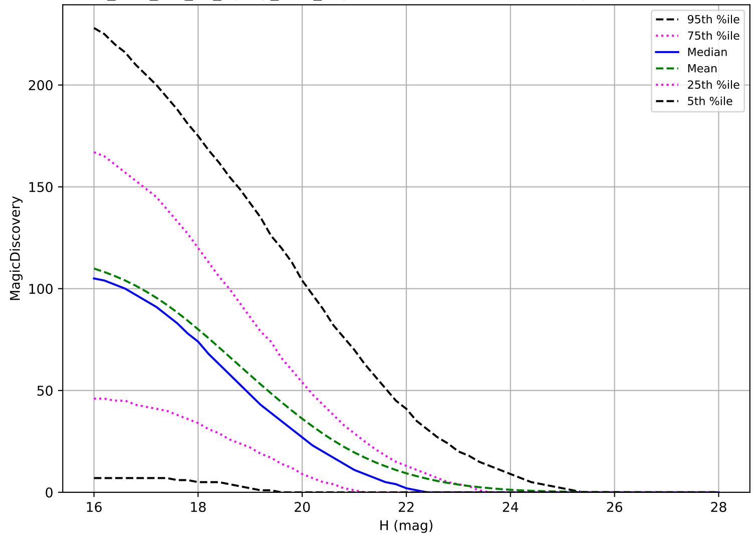
too_elab_r16_d3_ugrizy_v3.4_10yrs: PHA 6 detections in 60 nights detection loss
