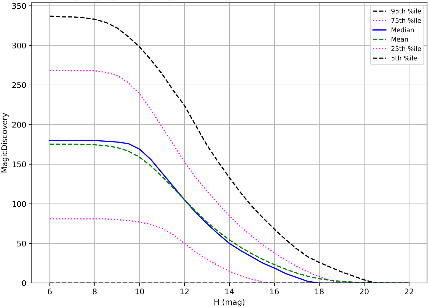
too_elab_r16_d3_ugrizy_v3.4_10yrs: OCC_r5 6 detections in 60 nights detection loss
