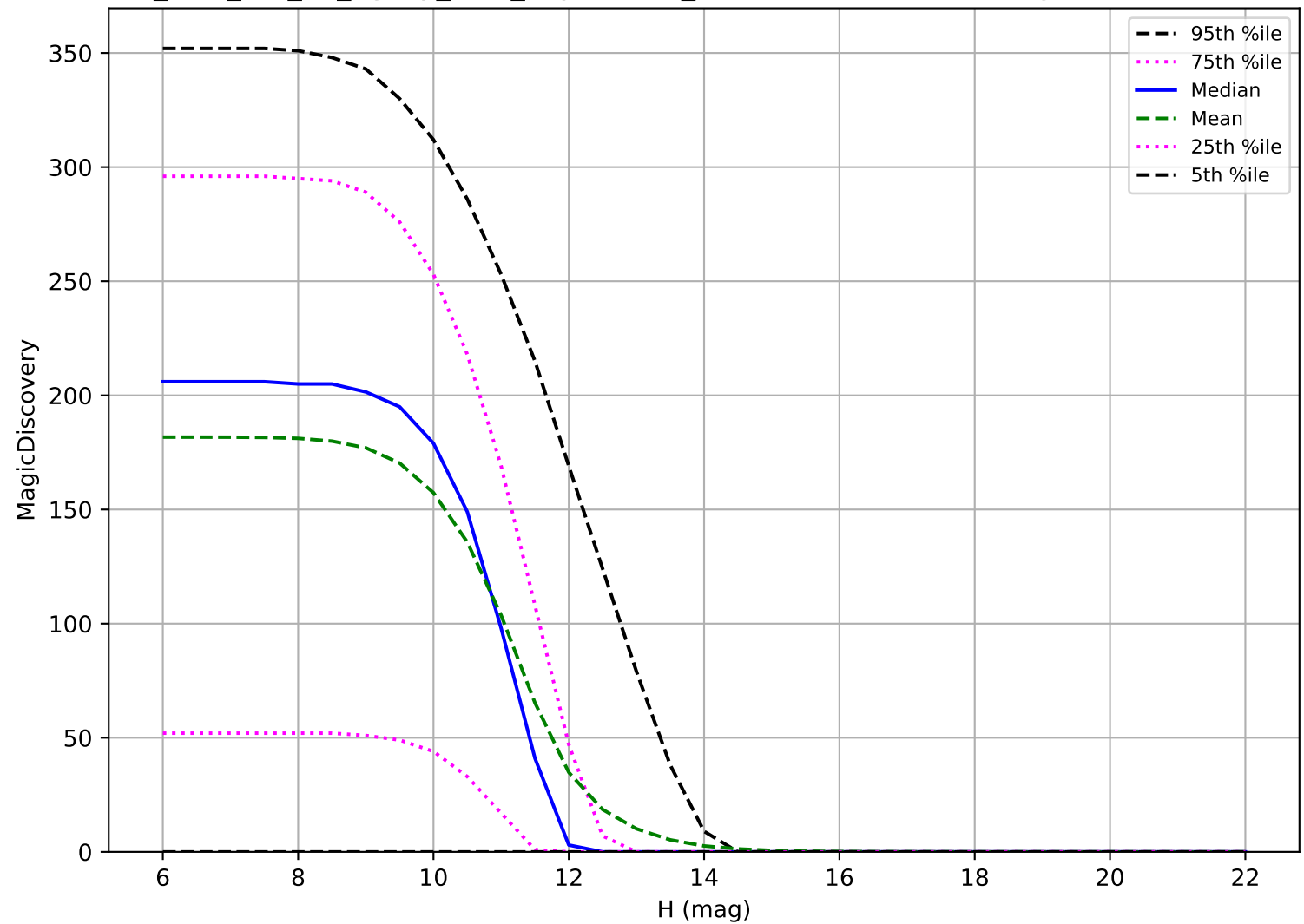
too_elab_r16_d3_ugrizy_v3.4_10yrs: OCC_r20 6 detections in 60 nights detection loss
