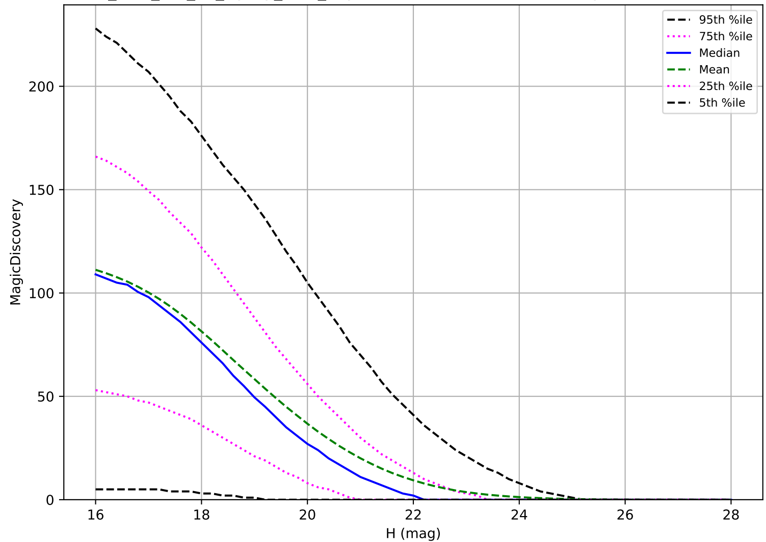
too_elab_r16_d3_ugrizy_v3.4_10yrs: NEO 6 detections in 60 nights detection loss
