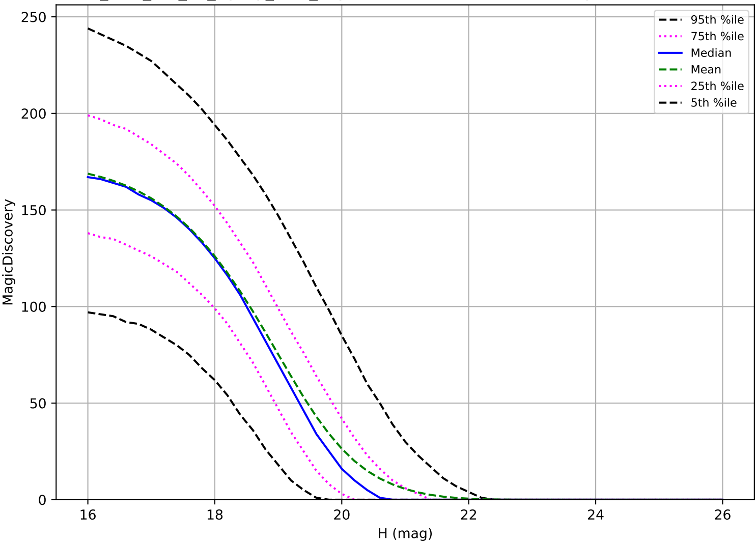
too_elab_r16_d3_ugrizy_v3.4_10yrs: MBA 6 detections in 60 nights detection loss
