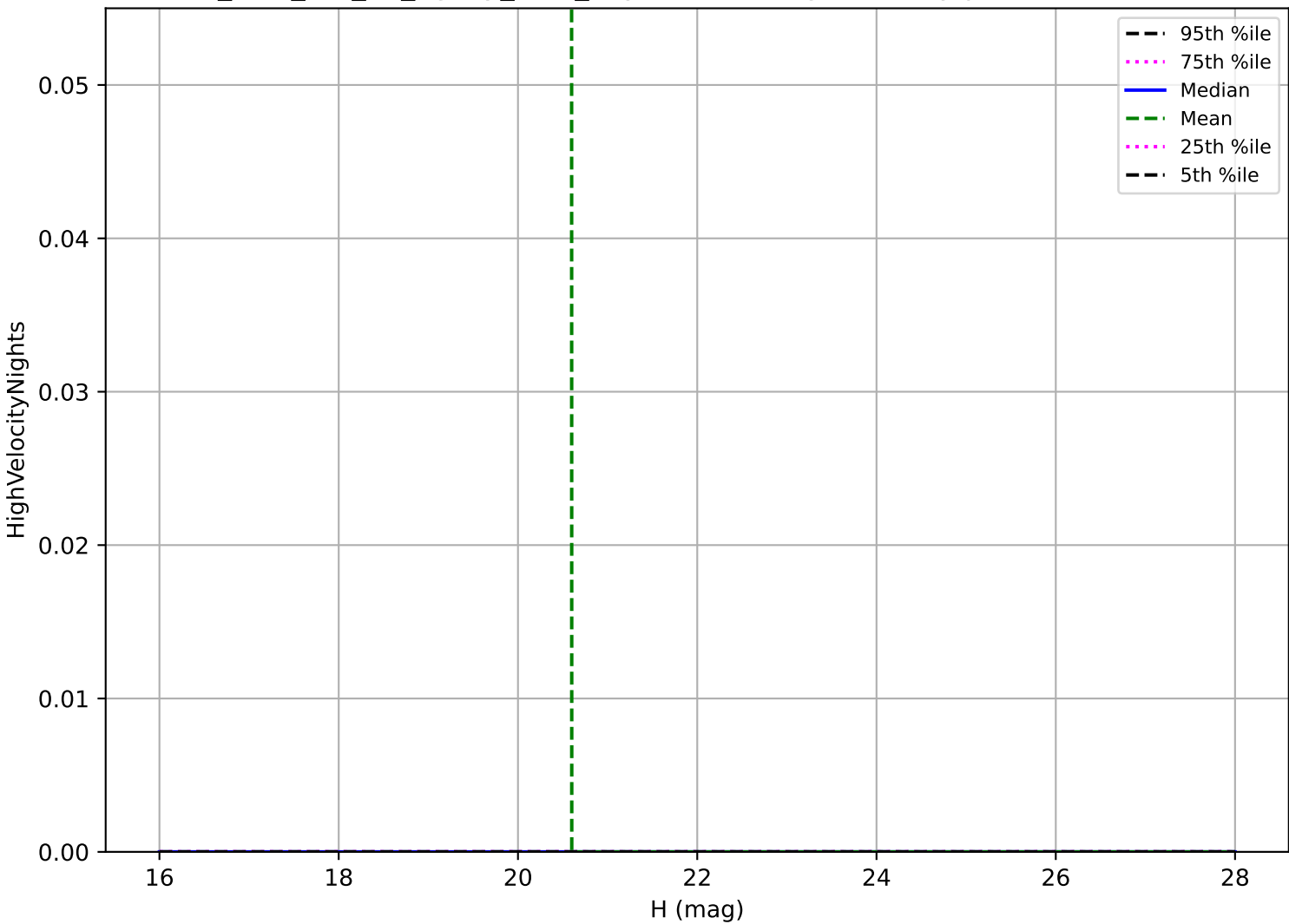
too_elab_r16_d3_ugrizy_v3.4_10yrs: Vatira High velocity pair detection loss
