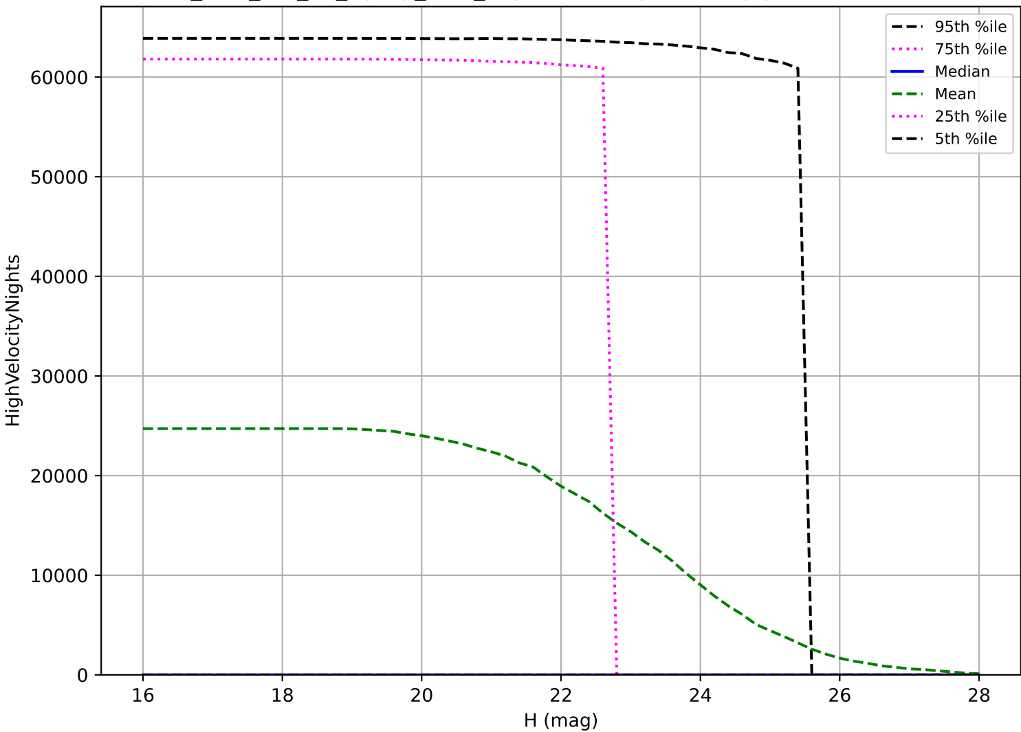
too_elab_r16_d3_ugrizy_v3.4_10yrs: PHA High velocity pair detection loss
