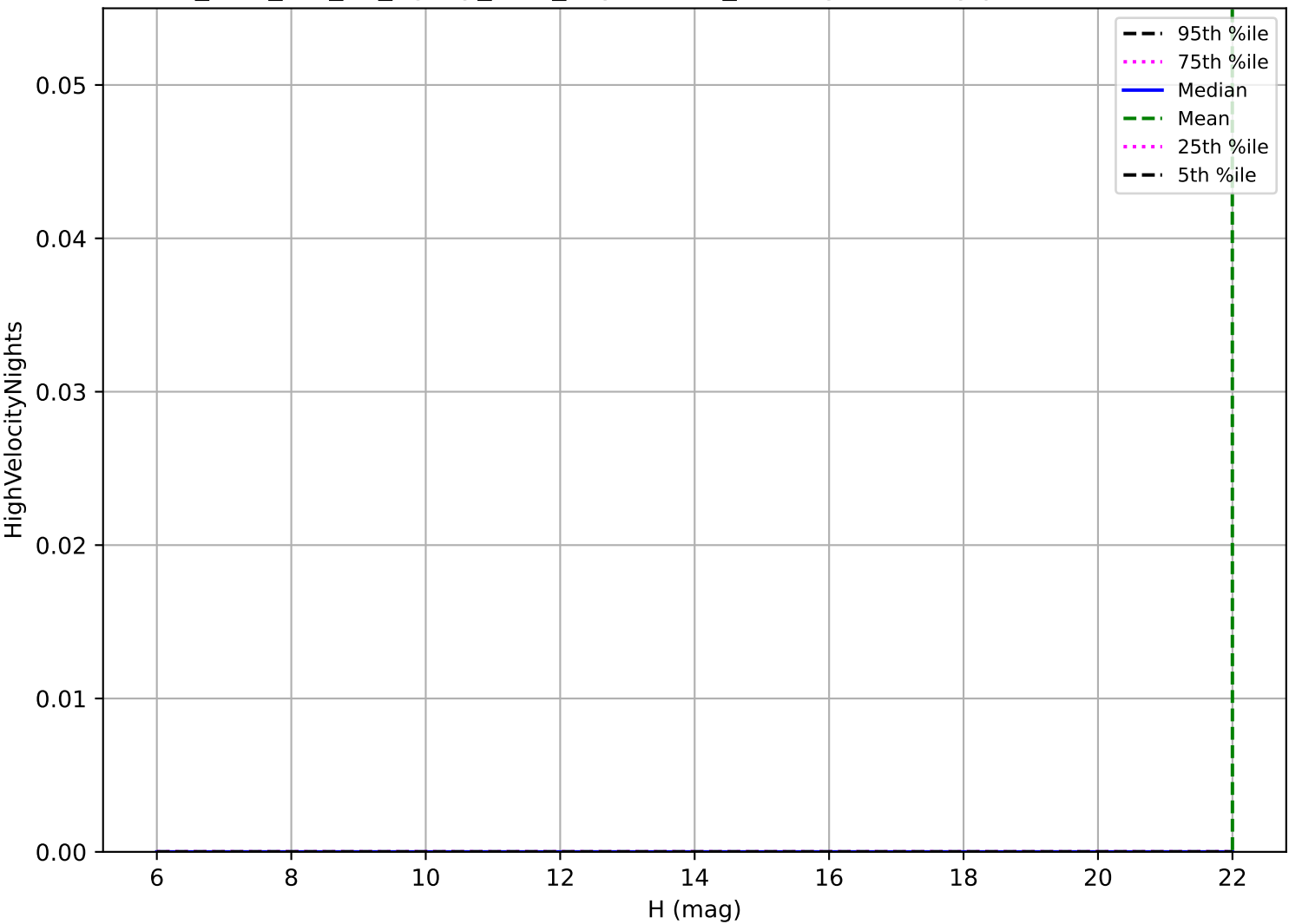
too_elab_r16_d3_ugrizy_v3.4_10yrs: OCC_r20 High velocity pair detection loss
