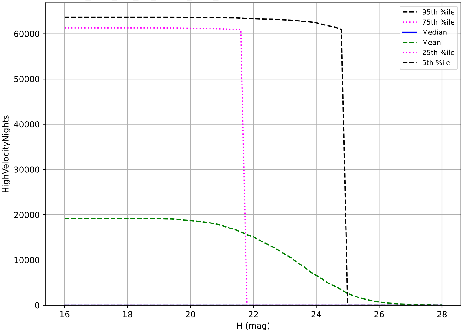
too_elab_r16_d3_ugrizy_v3.4_10yrs: NEO High velocity pair detection loss
