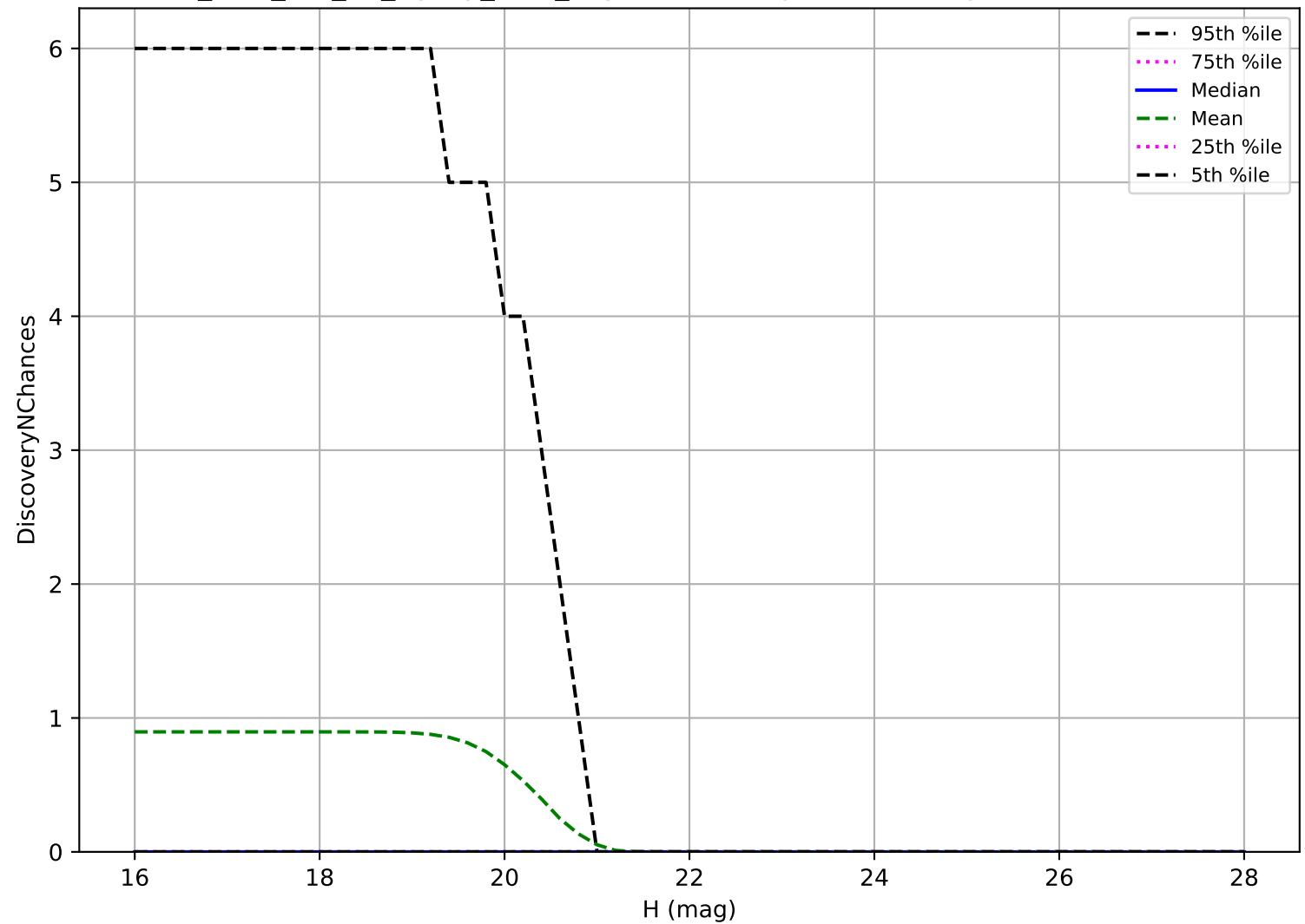
too_elab_r16_d3_ugrizy_v3.4_10yrs: Vatira 3 pairs in 15 nights detection loss
