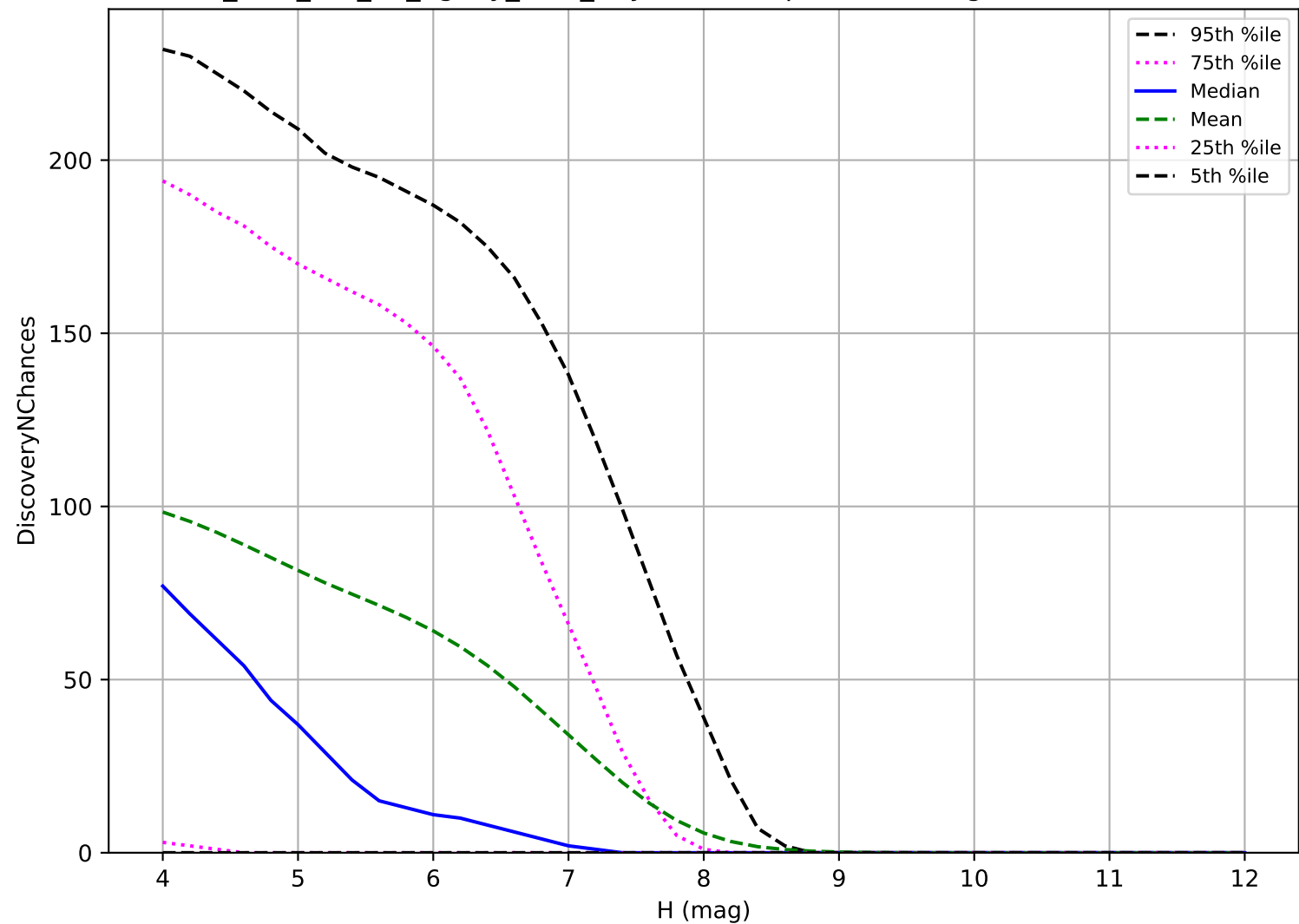
too_elab_r16_d3_ugrizy_v3.4_10yrs: TNO 3 pairs in 15 nights detection loss
