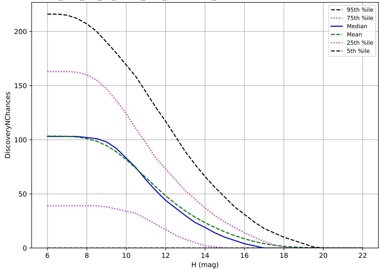
too_elab_r16_d3_ugrizy_v3.4_10yrs: OCC_r5 3 pairs in 15 nights detection loss
