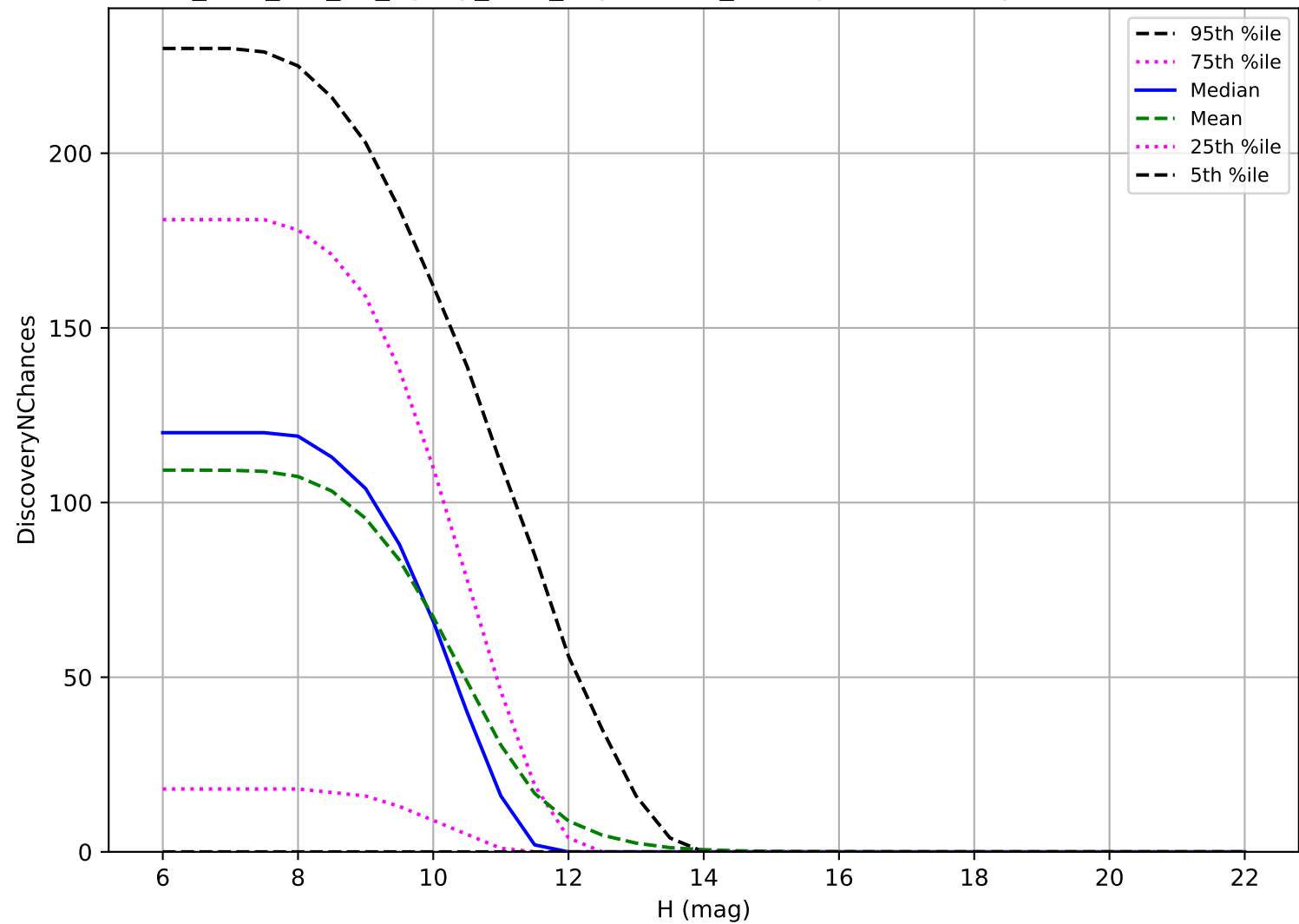
too_elab_r16_d3_ugrizy_v3.4_10yrs: OCC_r20 3 pairs in 15 nights detection loss
