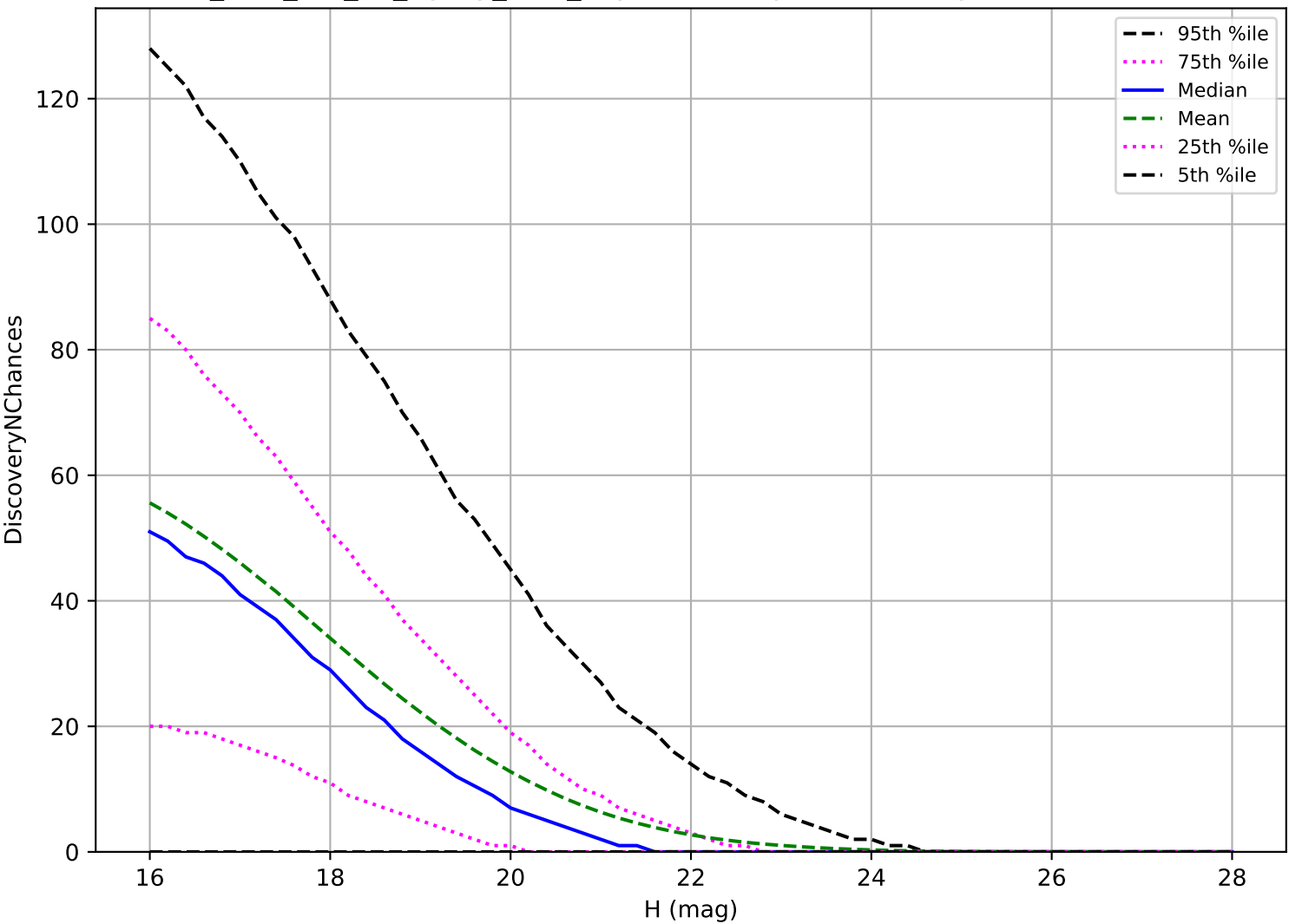
too_elab_r16_d3_ugrizy_v3.4_10yrs: NEO 3 pairs in 15 nights detection loss
