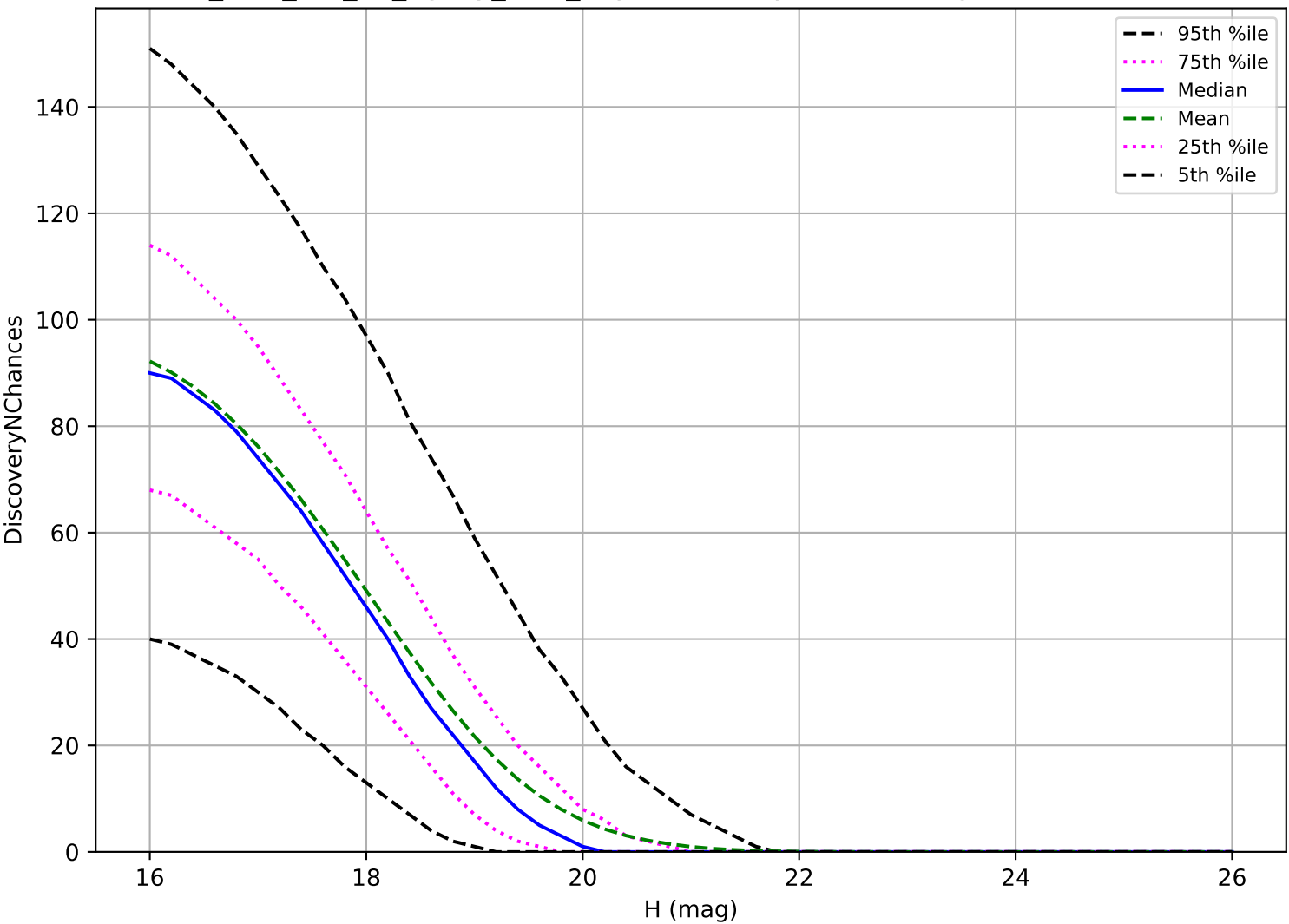
too_elab_r16_d3_ugrizy_v3.4_10yrs: MBA 3 pairs in 15 nights detection loss
