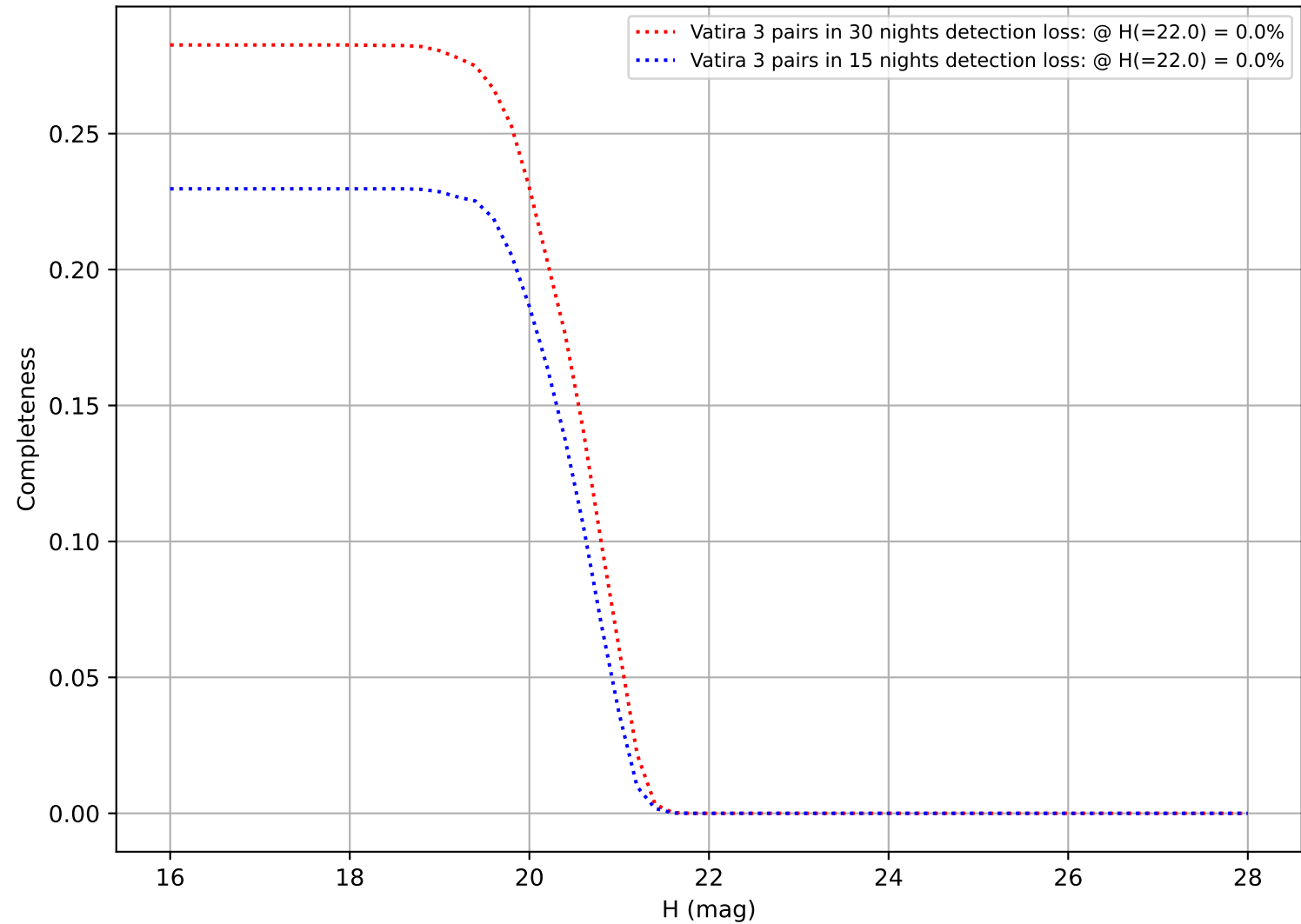
too_elab_r16_d3_ugrizy_v3.4_10yrs: DifferentialCompleteness
