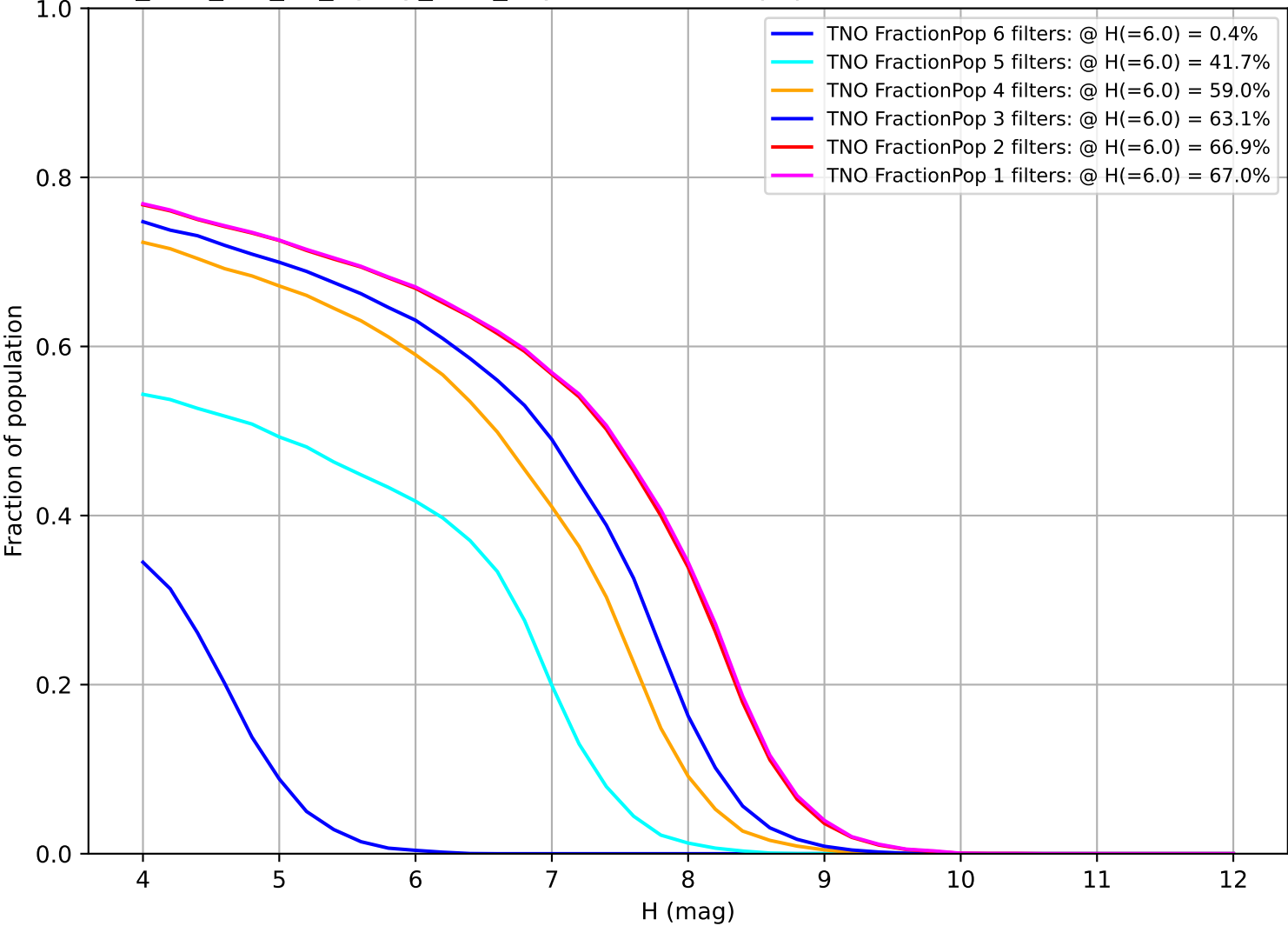
too_elab_r16_d3_ugrizy_v3.4_10yrs: Fraction of population with colors in X filters TNO
