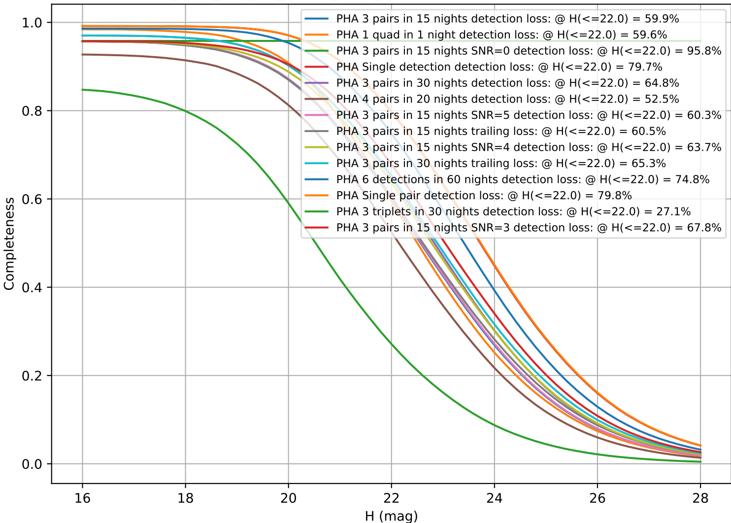
too_elab_r16_d3_ugrizy_v3.4_10yrs: CumulativeCompleteness
