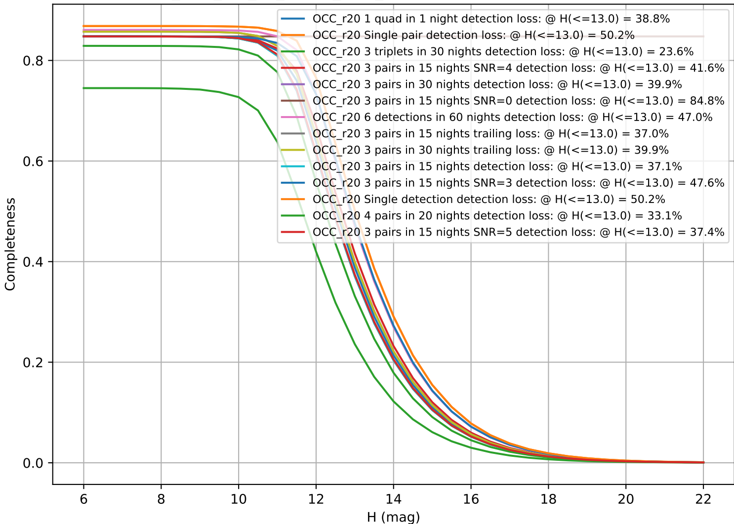
too_elab_r16_d3_ugrizy_v3.4_10yrs: CumulativeCompleteness
