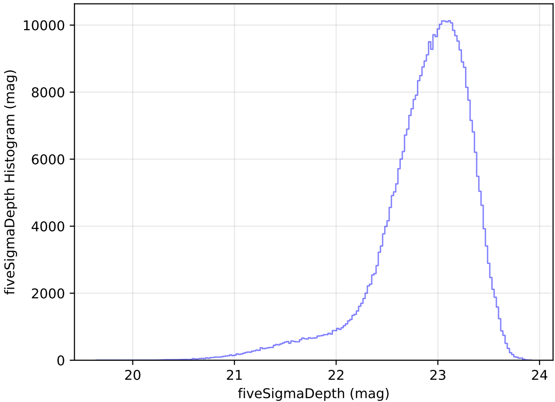
too_elab_r16_d3_ugrizy_v3.4_10yrs z: fiveSigmaDepth Histogram
