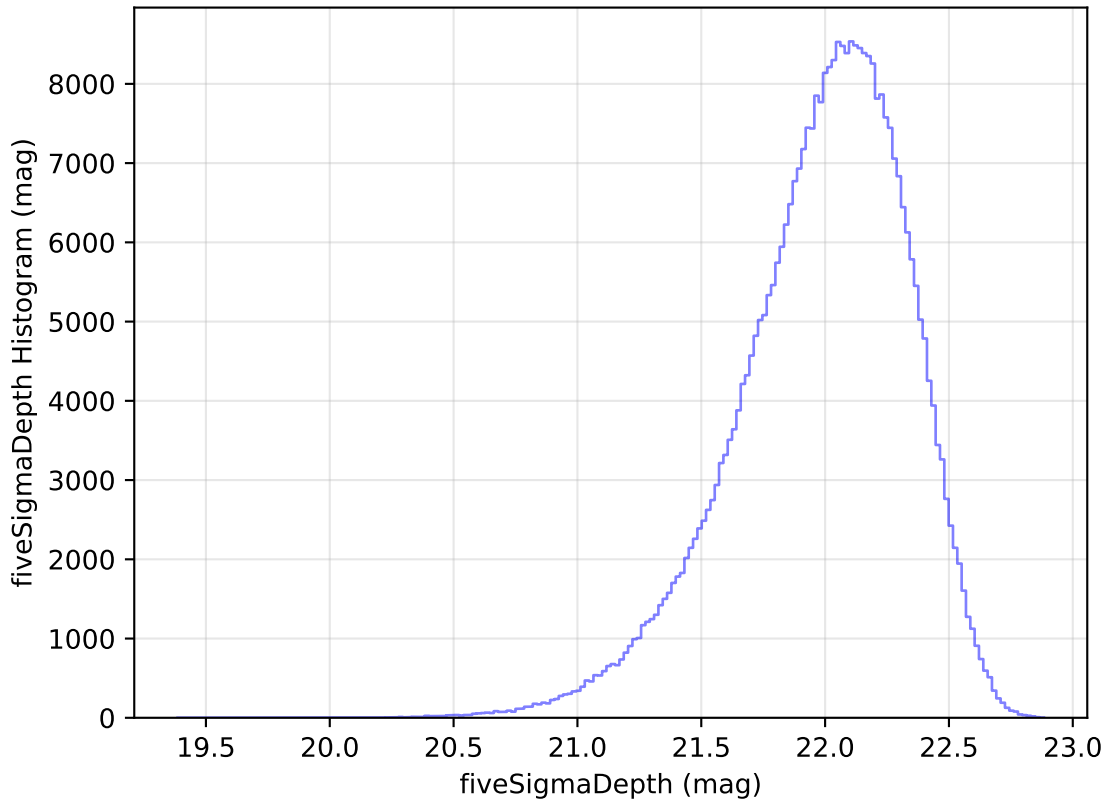
too_elab_r16_d3_ugrizy_v3.4_10yrs y: fiveSigmaDepth Histogram
