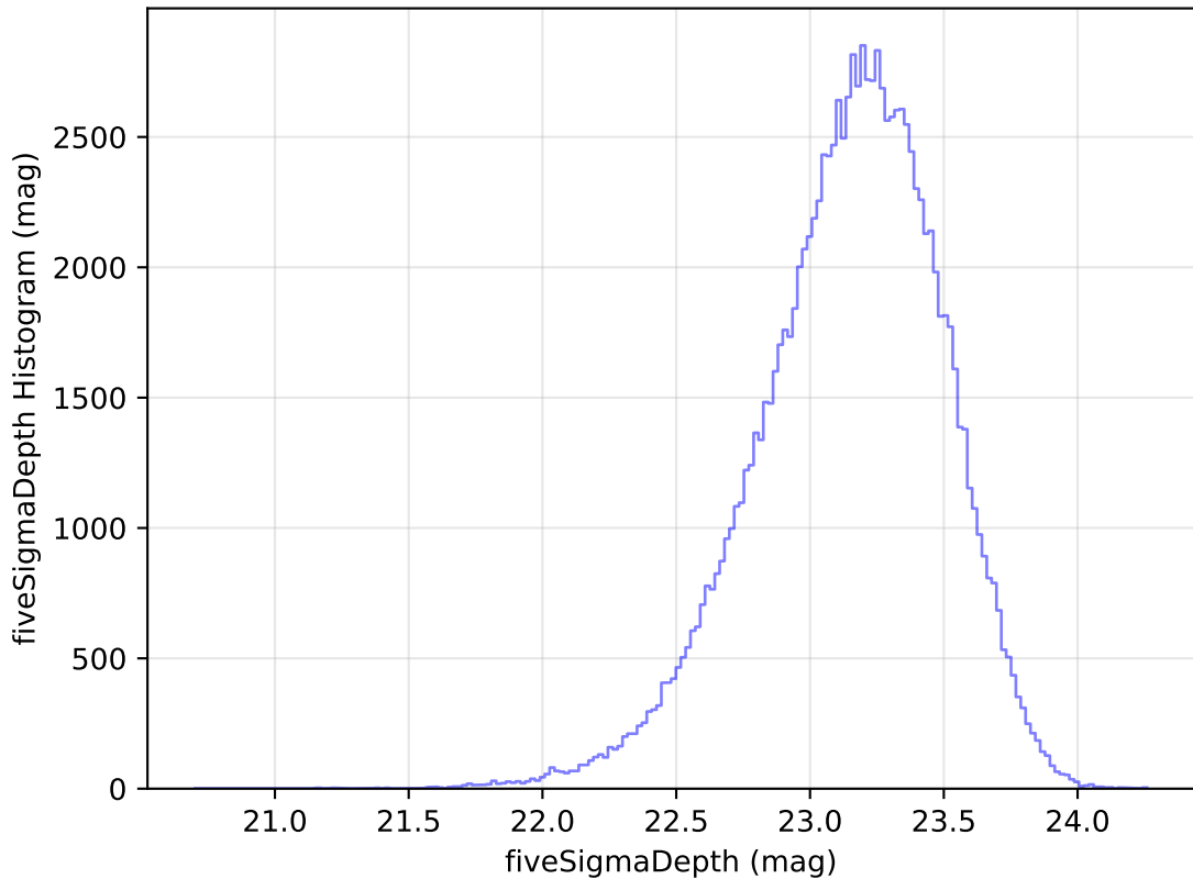
too_elab_r16_d3_ugrizy_v3.4_10yrs u: fiveSigmaDepth Histogram
