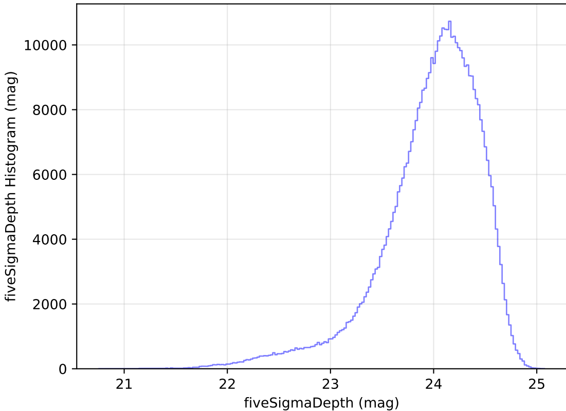
too_elab_r16_d3_ugrizy_v3.4_10yrs r: fiveSigmaDepth Histogram
