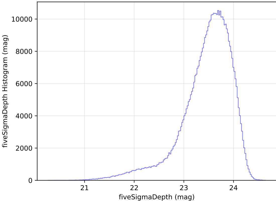
too_elab_r16_d3_ugrizy_v3.4_10yrs i: fiveSigmaDepth Histogram
