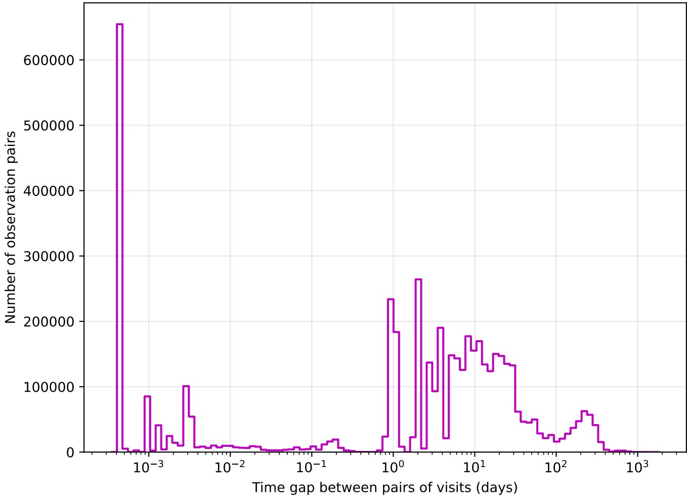
too_elab_r16_d3_ugrizy_v3.4_10yrs z band: Tgaps observationStartMJD
