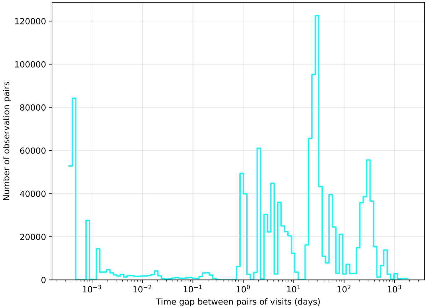
too_elab_r16_d3_ugrizy_v3.4_10yrs u band: Tgaps observationStartMJD
