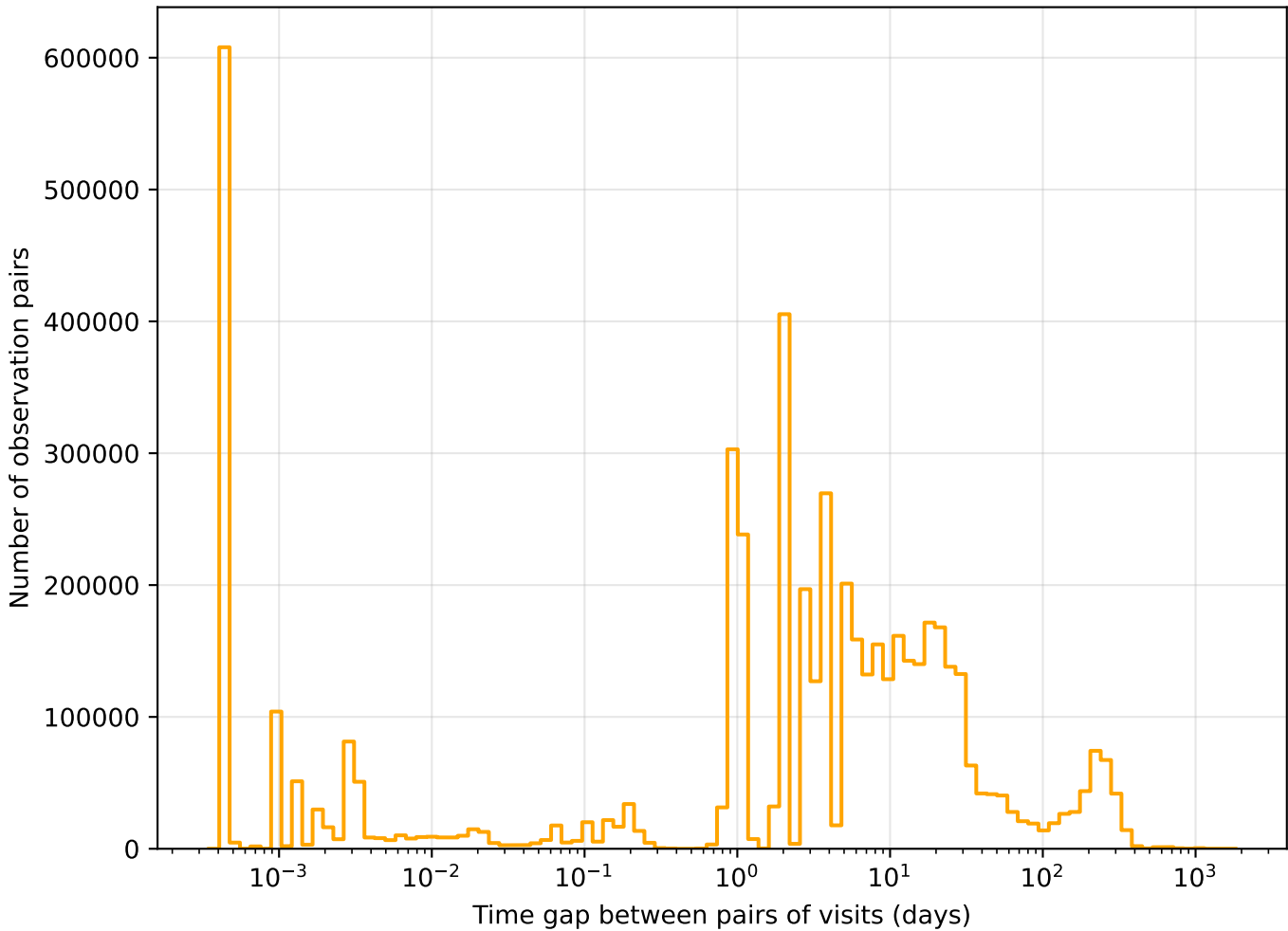
too_elab_r16_d3_ugrizy_v3.4_10yrs r band: Tgaps observationStartMJD
