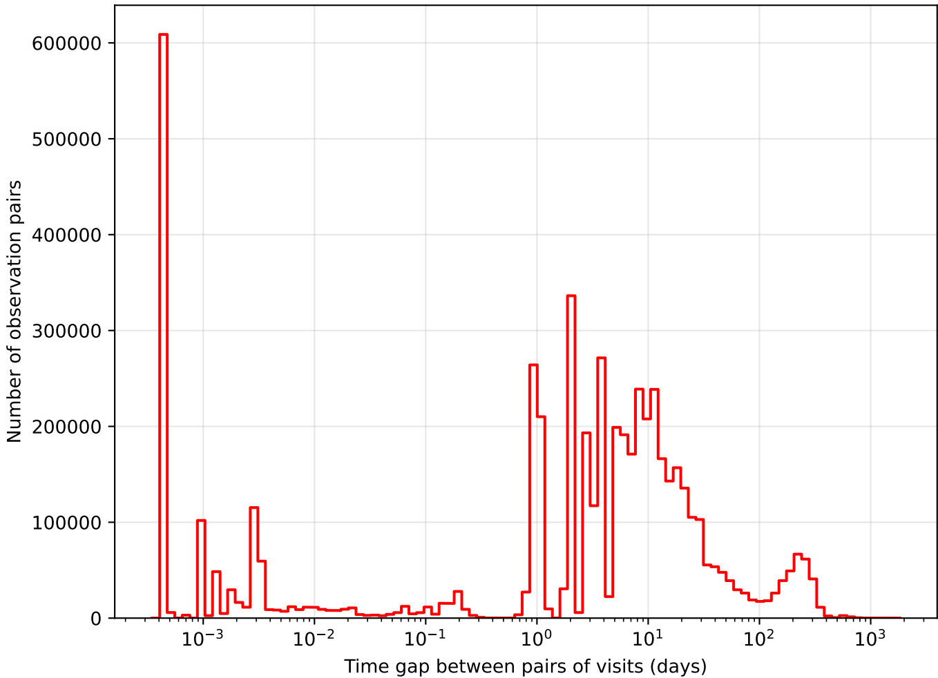
too_elab_r16_d3_ugrizy_v3.4_10yrs i band: Tgaps observationStartMJD
