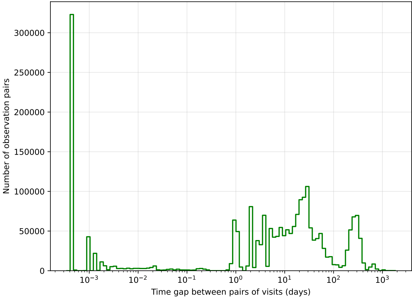
too_elab_r16_d3_ugrizy_v3.4_10yrs g band: Tgaps observationStartMJD
