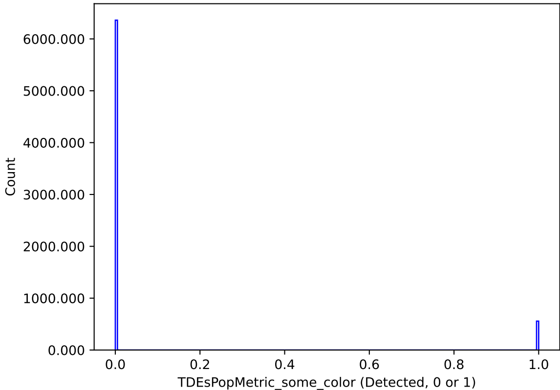
too_elab_r16_d3_ugrizy_v3.4_10yrs : TDEsPopMetric_some_color
