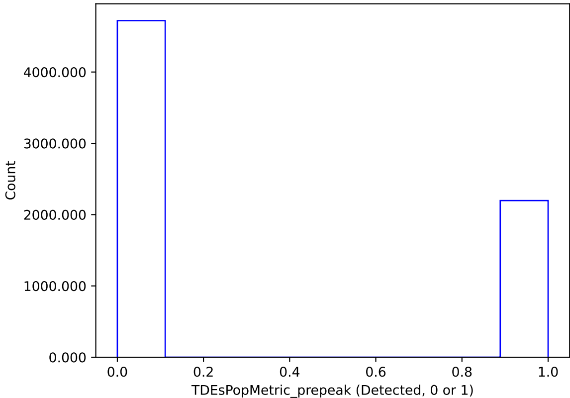
too_elab_r16_d3_ugrizy_v3.4_10yrs : TDEsPopMetric_prepeak
