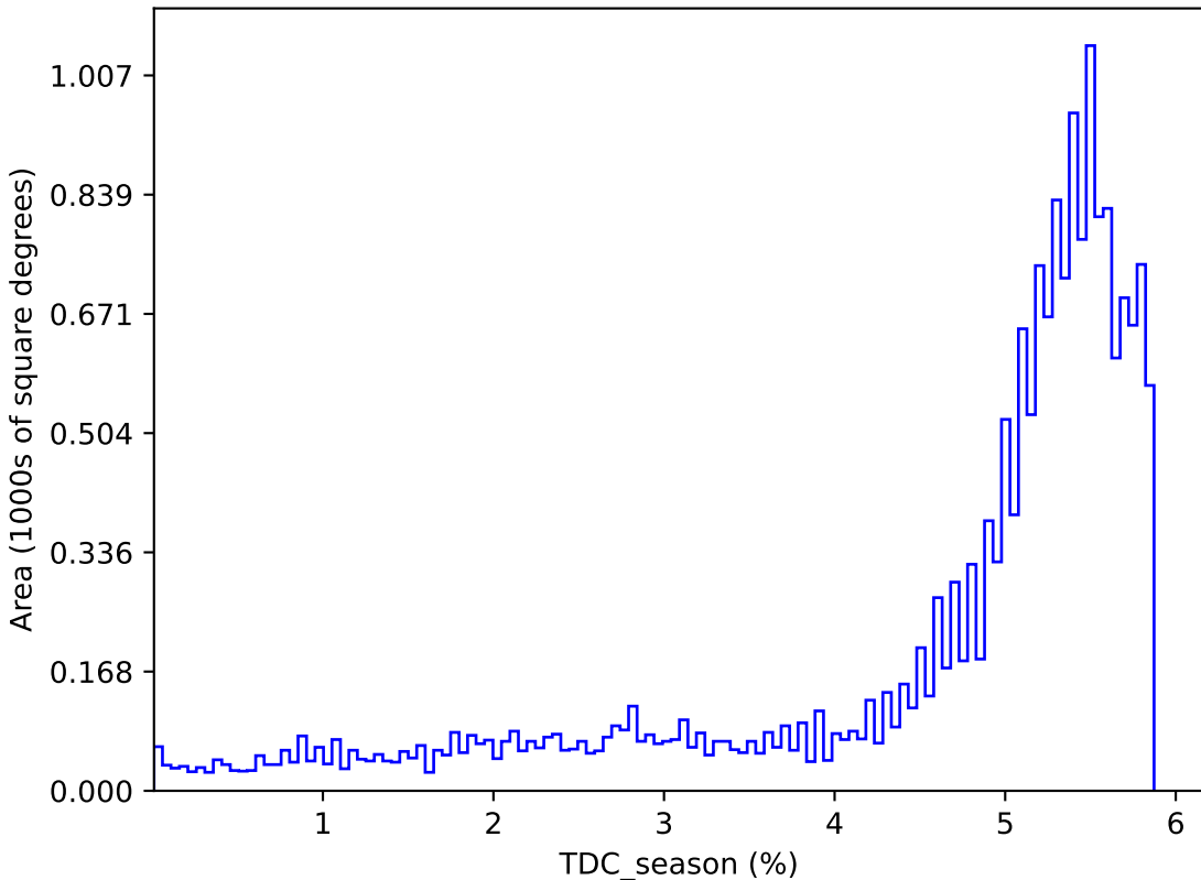
too_elab_r16_d3_ugrizy_v3.4_10yrs : TDC_season
