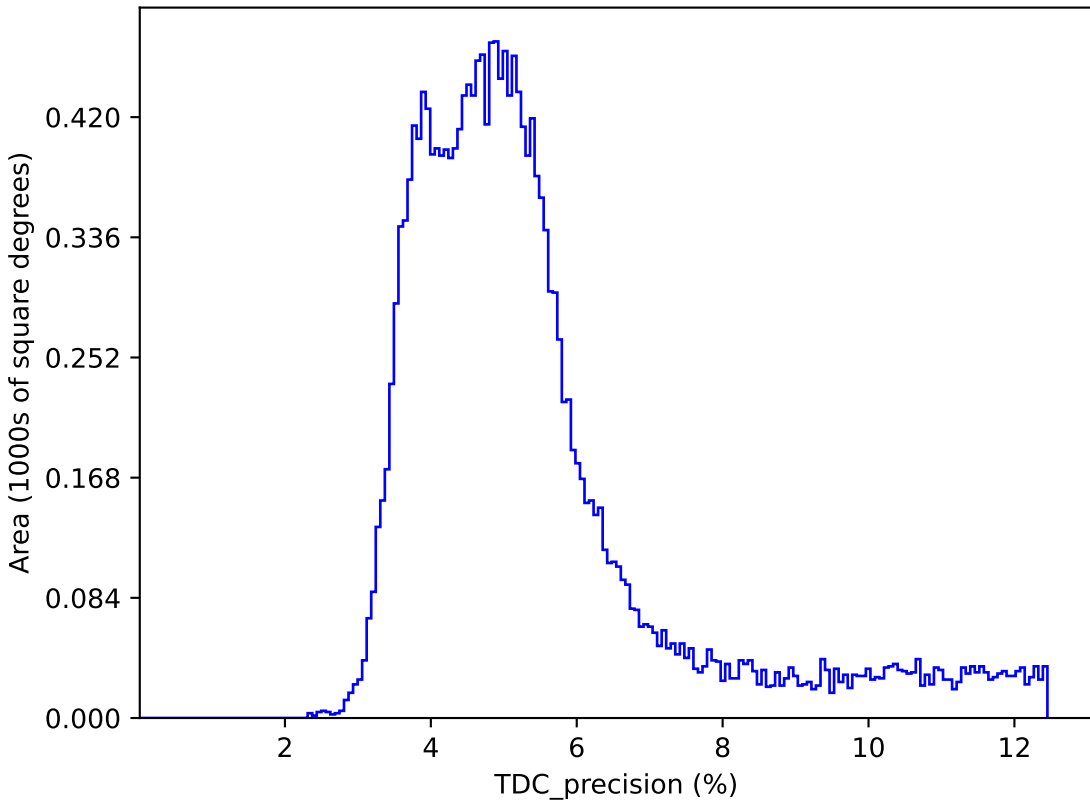
too_elab_r16_d3_ugrizy_v3.4_10yrs : TDC_precision
