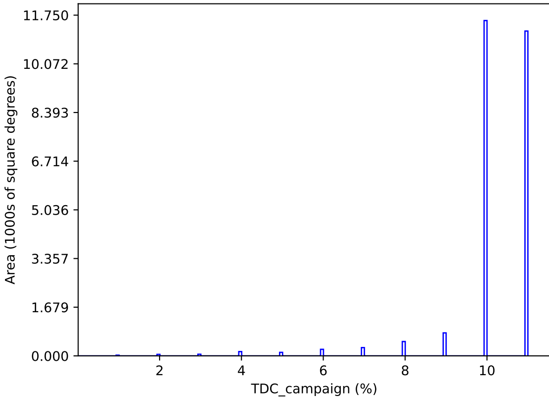
too_elab_r16_d3_ugrizy_v3.4_10yrs : TDC_campaign
