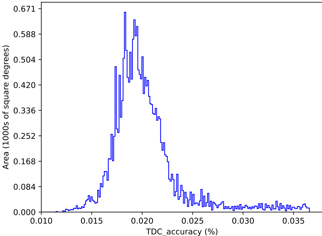
too_elab_r16_d3_ugrizy_v3.4_10yrs : TDC_accuracy
