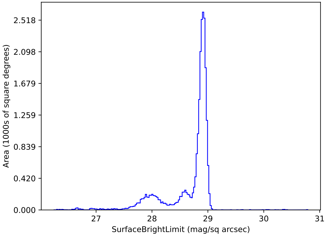
too_elab_r16_d3_ugrizy_v3.4_10yrs u: SurfaceBrightLimit
