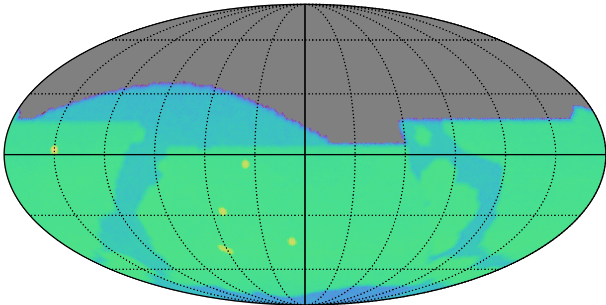
too_elab_r16_d3_ugrizy_v3.4_10yrs r: SurfaceBrightLimit
